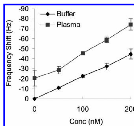
Figure 2. Calibration plot obtained with different concentrations of thrombin in buffer and plasma.
